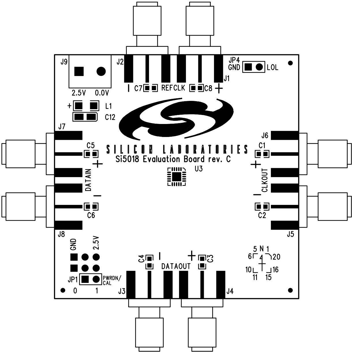
Figure 3. Si5018 Silkscreen
