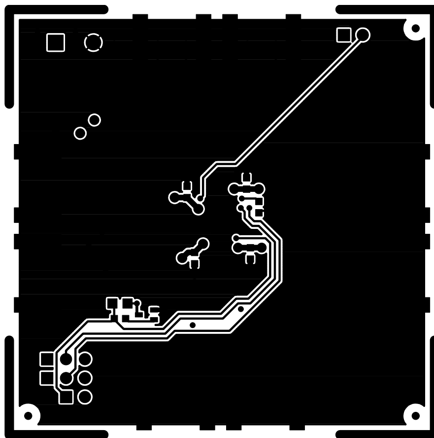
Figure 5. Solder Side
